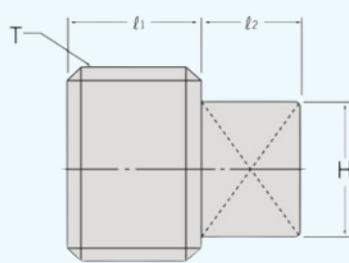
Square Plug
