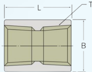
Full Coupling
