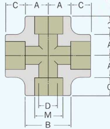
Cross
