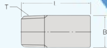
Round Plug
