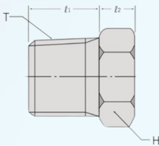
Hex. Head Plug
